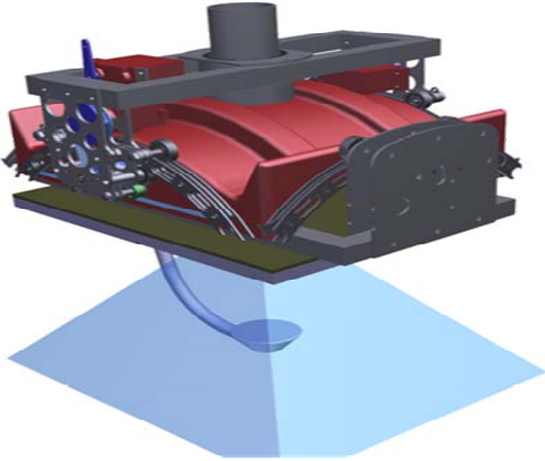
Fig. 5. Electromechanical stabilization unit.
