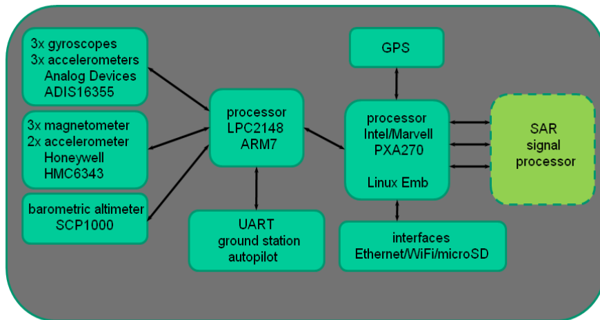
Fig. 7. AHRS unit design [4].
