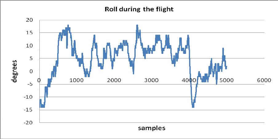
Fig. 2. Roll during the flight mission.
